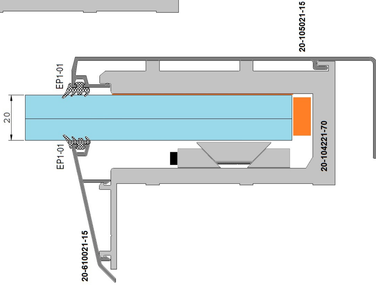
Variant 2: 20 mm glass
