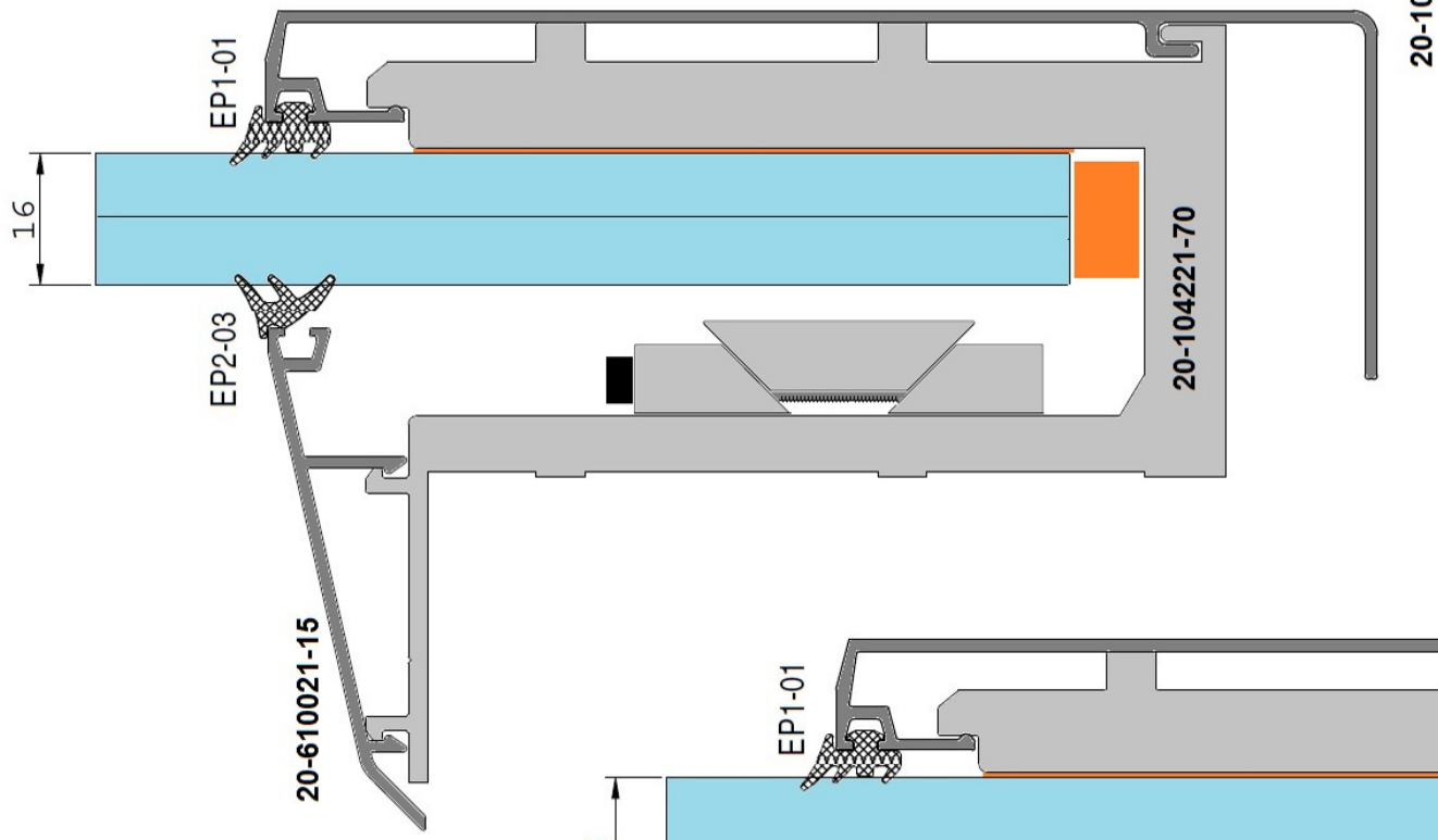
Variant 1: 16 mm glass
